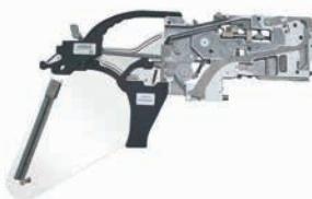
SM 8X4 FEEDER
